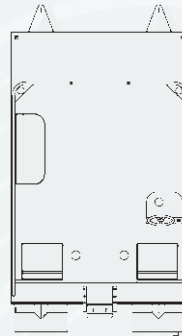
Angler - Floor Plan Includes steering console, 2 rear seats and built-in livewell box with integrated cushions
